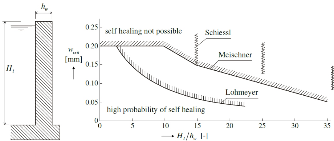
Figure 2 Lohmeyer's table (after [3])
